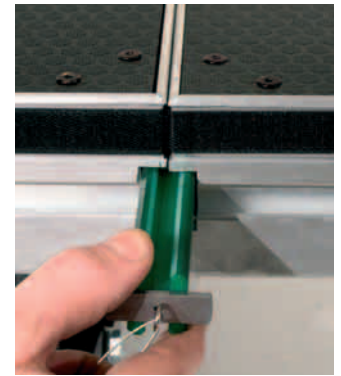
Linking CFP.LNK
